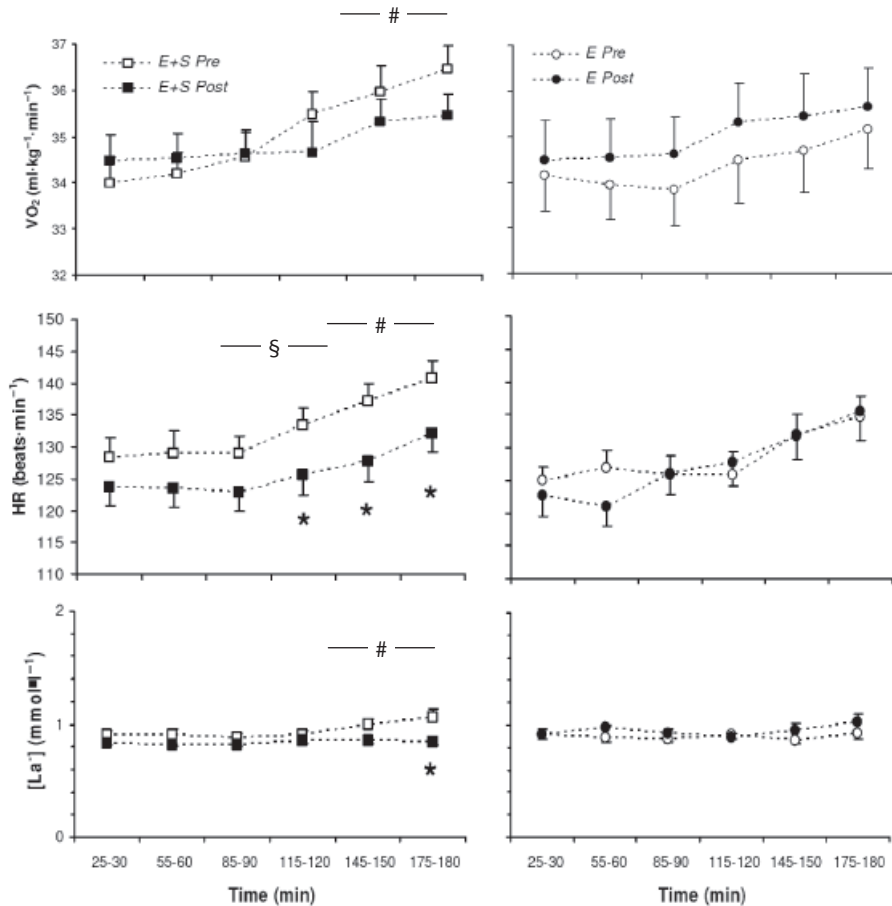
Fig. 2. Oxygen uptake ( \text{VO}_2 ; top), heart rate (HR; mid) and blood lactate concentration ( [\text{La}^-] ; bottom) during 180 min of cycling at 44% of baseline W_{\text{max}} before (Pre) and after (Post) 12 weeks of concurrent endurance (cycling) and strength training (E+S; left) and endurance (cycling) training alone (E; right). W_{\text{max}} was calculated as the mean power output during the final 2 min of a short-term all-out incremental \text{VO}_{2\text{max}} test. *Post different from pre ( P < 0.05 ), relative changes (pre-to-post training) different between E+S and E at 120–180 min (#, P < 0.01 ) and 60–120 min (§, P < 0.01 ). Data adapted from Rønnestad et al. (2010).
